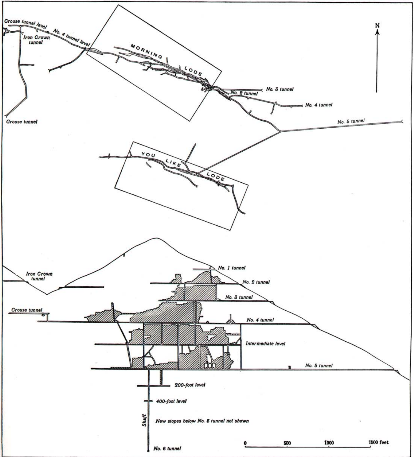
PLAN OF UNDERGROUND WORKINGS OF MORNING MINE, WITH A LONGITUDINAL VERTICAL PROJECTION OF THE WORKINGS ON THE MORNING LODE.
