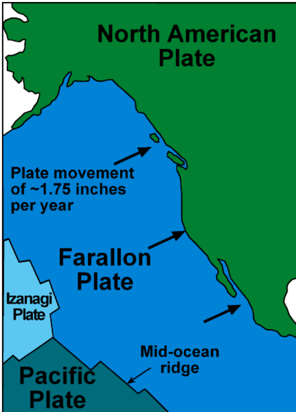
100 Ma (Middle Cretaceous) Plate tectonic configuration. Redrawn from Orr and Orr (2002).
